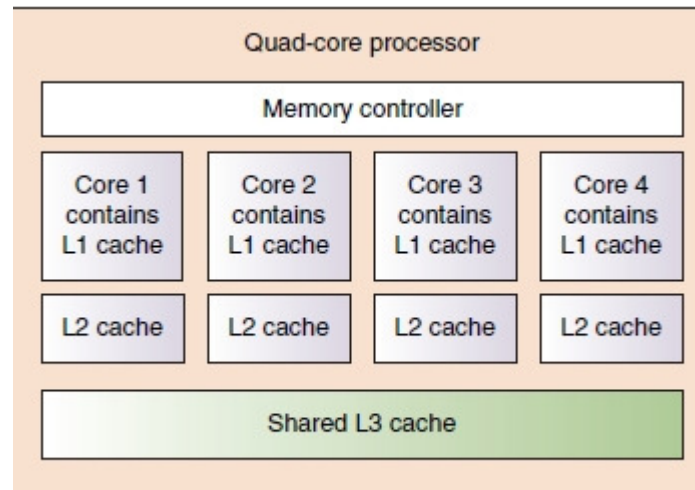
Figure 6-4 Quad-core processing with L1, L2, and L3 cache and the memory controller within the processor housing
