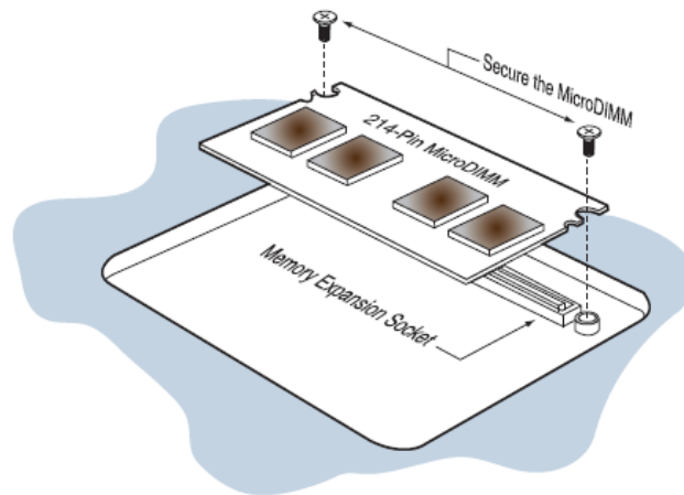
Figure 21-45 Installing a MicroDIMM in a subnotebook computer Courtesy: Course Technology/Cengage Learning
